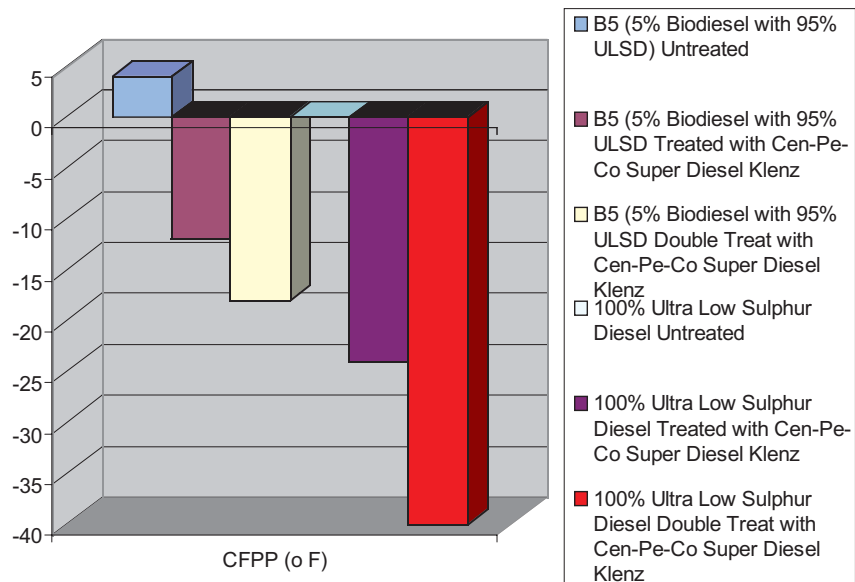
Cold Filter Plugging Point Tests With and Without Additive
